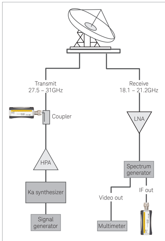
Typical satellite test system set-up
